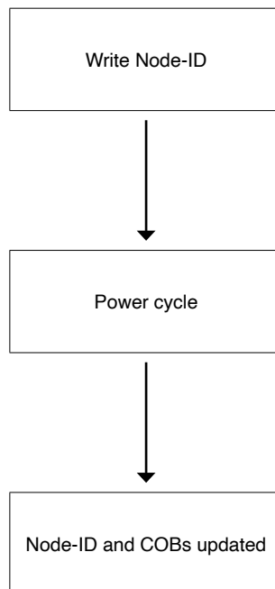
Figure 39 - Setting Node-ID by SDO write
