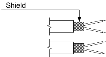
2x PVC screened cable (standard); 2 x 0.14 mm \varnothing ; \varnothing 3.5mm
