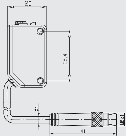
M8 connector
